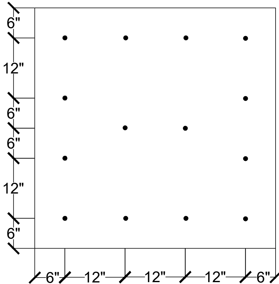
14 FASTENERS PER 4' x 4' BOARD
