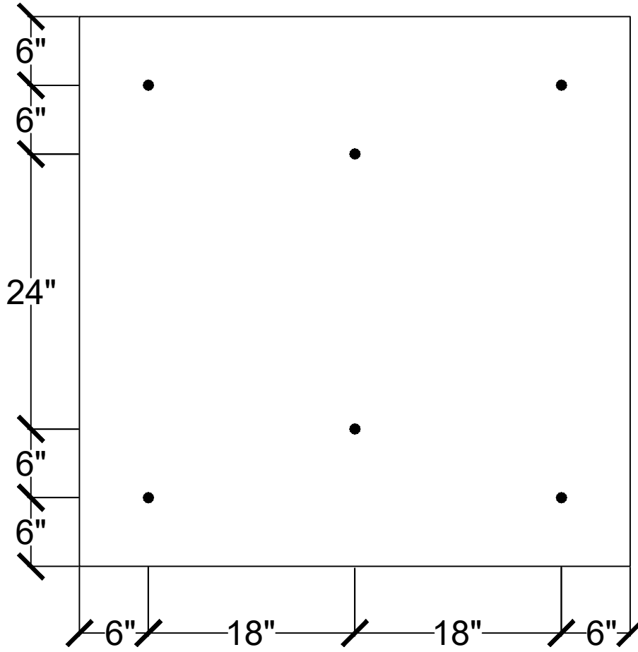
6 FASTENERS PER 4' x 4' BOARD
